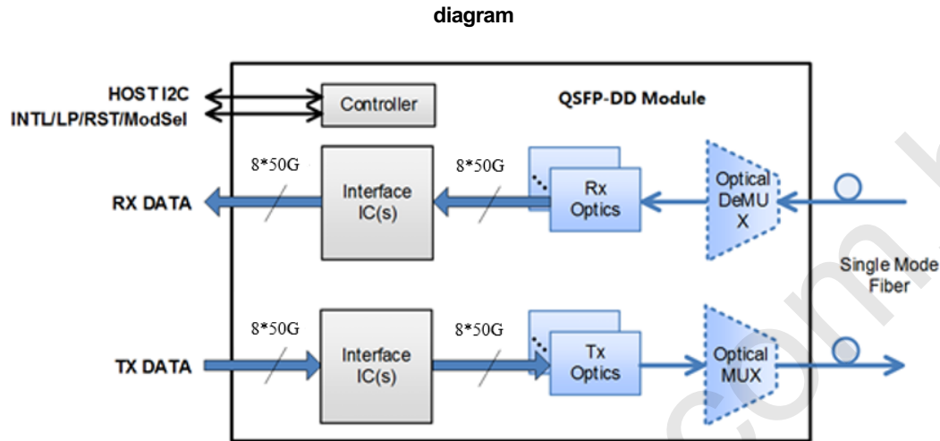
Figure 1-3 Transceiver block
