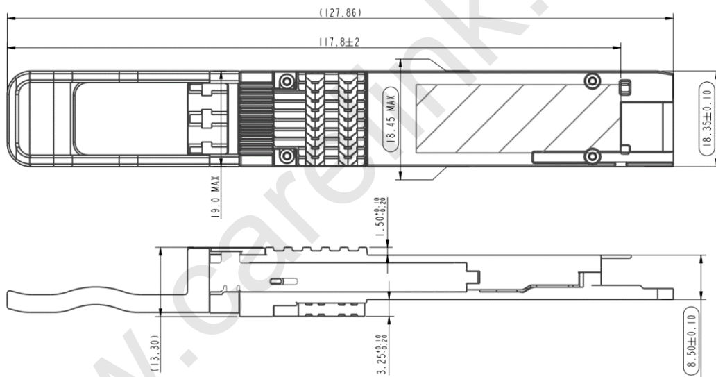
Figure 1-2 Mechanical dimensions
