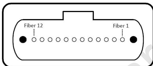
Outside View of the QSFP Module MPO
