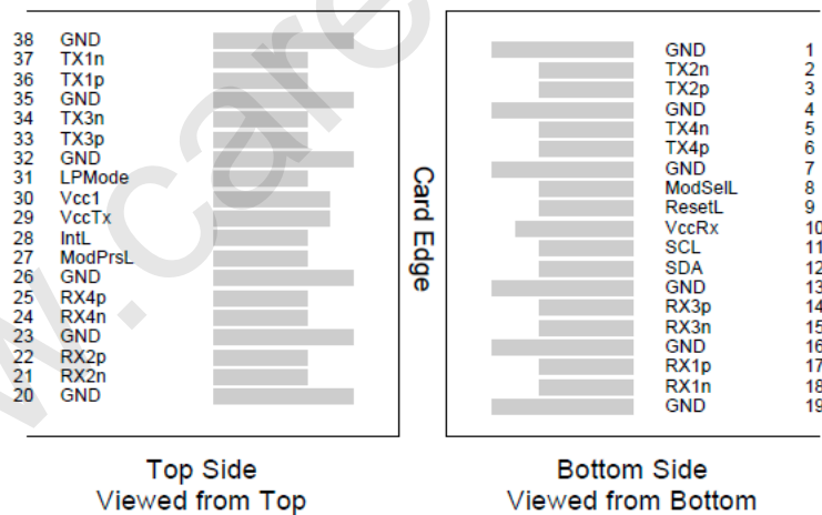
QSFP Transceiver Pad Layout
