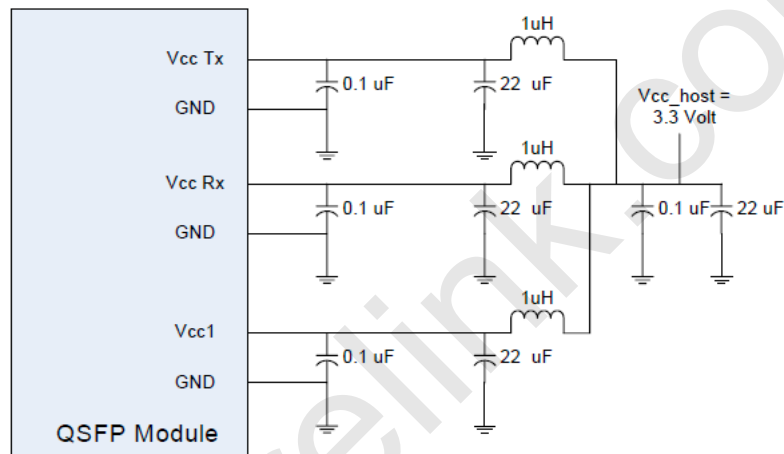
Recommended Host Board Power Supply Filtering
