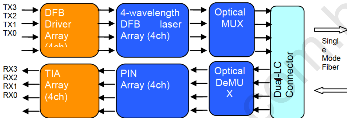
Figure 1: 40Gb/s QSFP IR4 Transceiver Block Diagram
