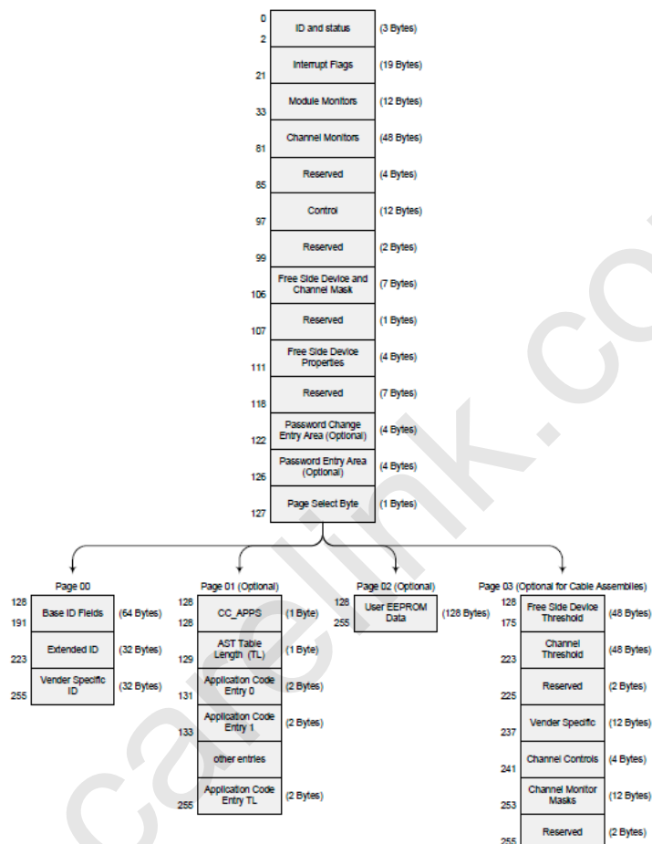
QSFP Memory Map
