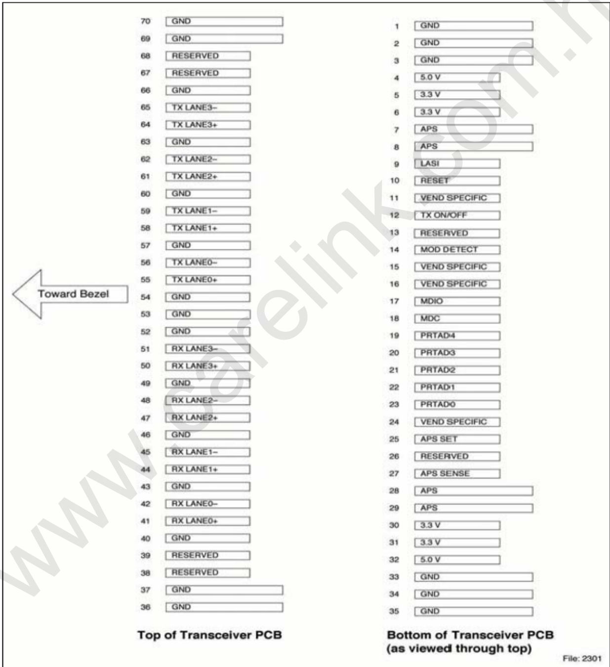
Fig 1-XENPAK Transponder Electrical Pad Layout
