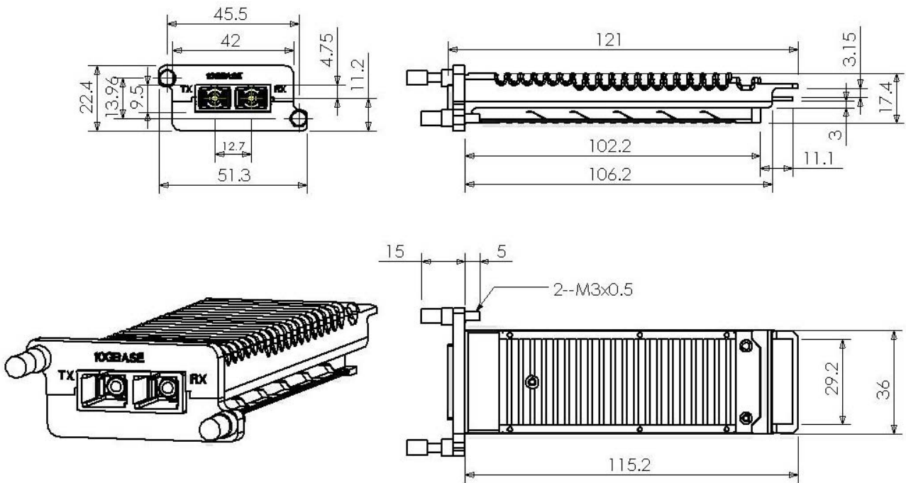
Figure 1 Mechanical dimensions
