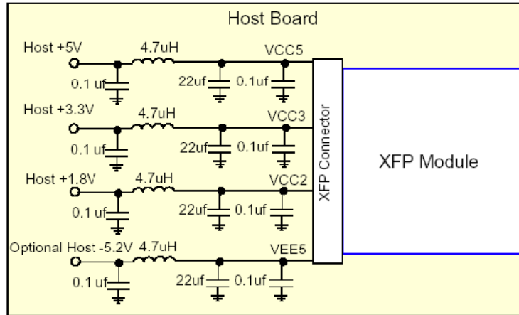
Recommended Host Board Power Supply Circuit
