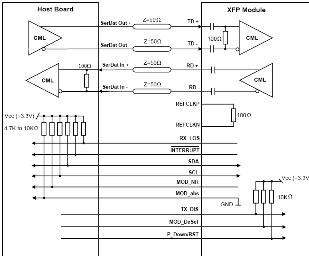
Recommended High-speed Interface Circuit
