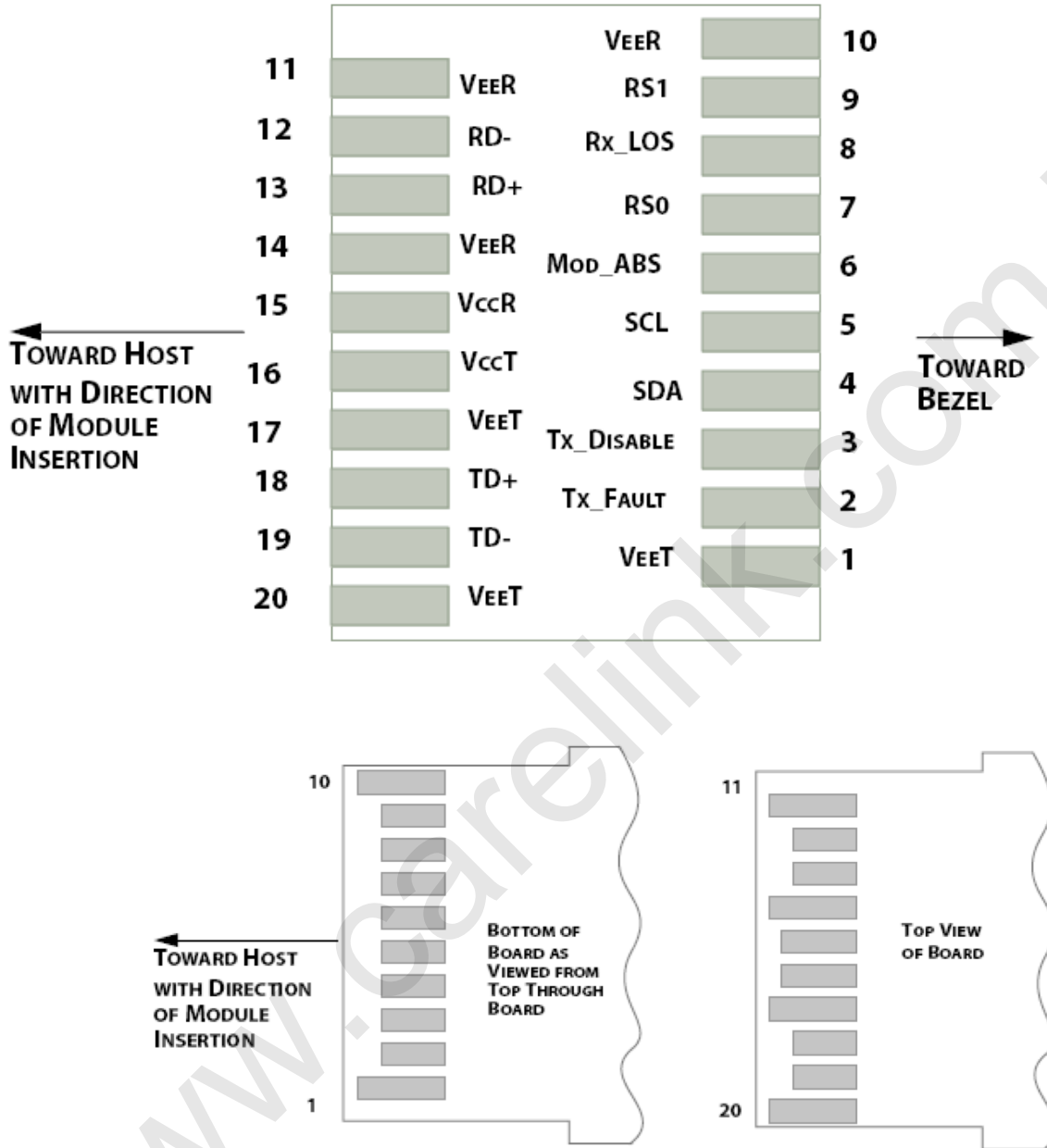
Figure2.Electrical Pin-out Details
