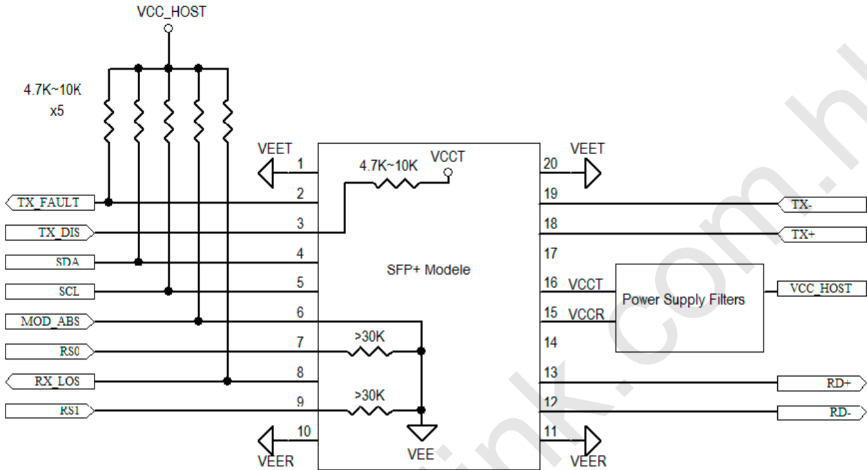
Figure4. Host-Module Interface
