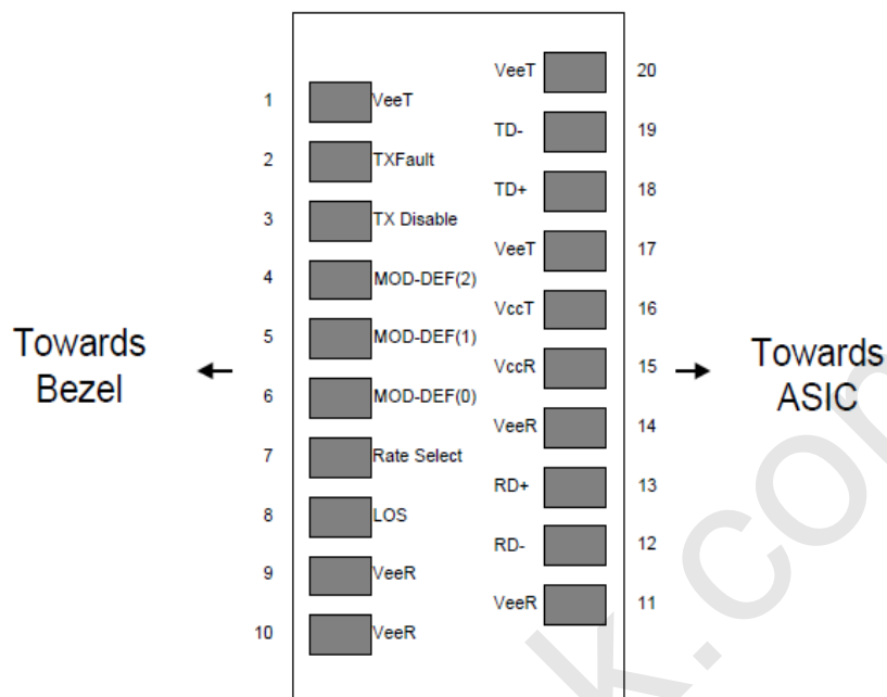
Figure 1. Diagram of host board connector block pin numbers and name+3.3V VOLT ELECTRICAL POWER INTERFACE The SFP+-10GBASE-T has an input voltage range of 3.3 V +/- 5%. The 4Vmaximum voltage is not allowed for continuous operation.
