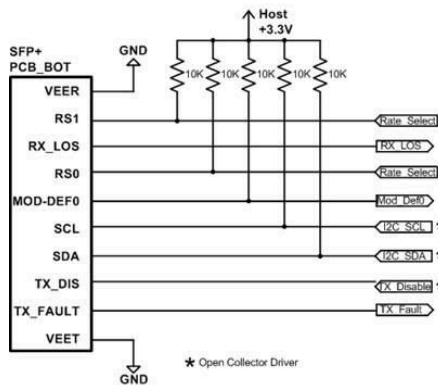
Recommended High-speed Interface Circuit
