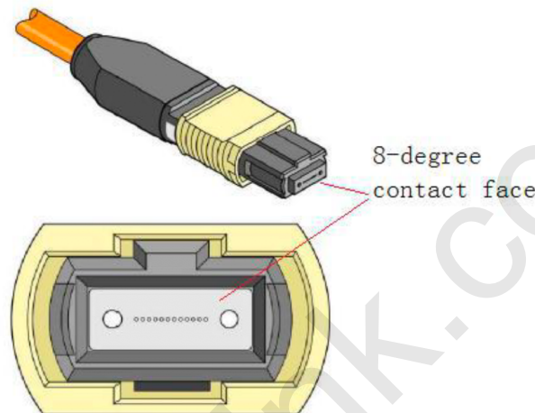
Figure 5. Female MPO Connector with 8-degree End-face
